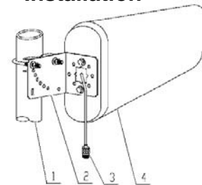
Pole holding installation
