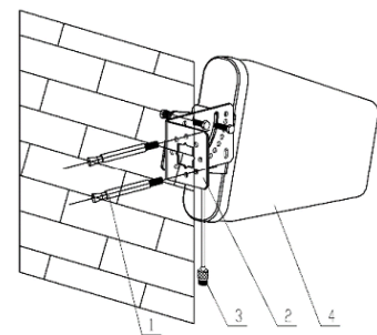
Wall mounting installation
